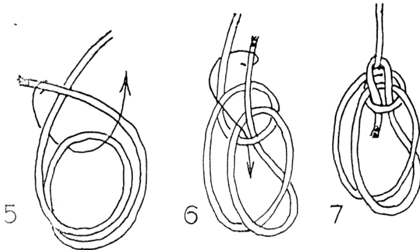
PORTUGUESE BOWLINE
