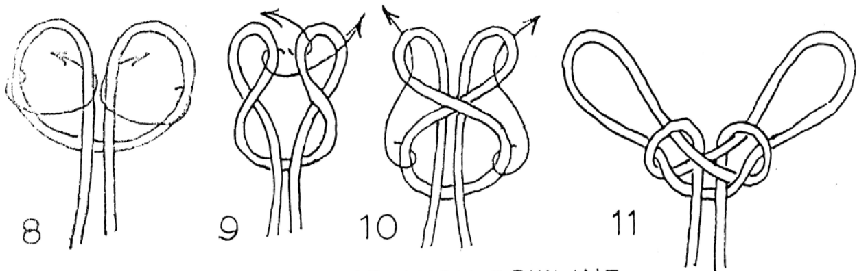
SPANISH BOWLINE
